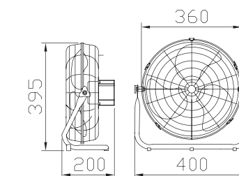
FE-30B
