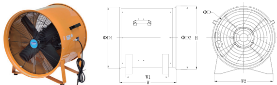
PVT-45(18"),PVT-50(20"),PVT-60(24")Structure
