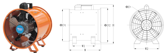
PVT20(8"),PVT-25(10"),PVT-30(12"),PVT-35(14"),PVT-40(16")Structure
