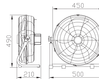
FE-40B
