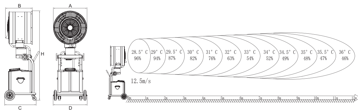
Outline dimensions
