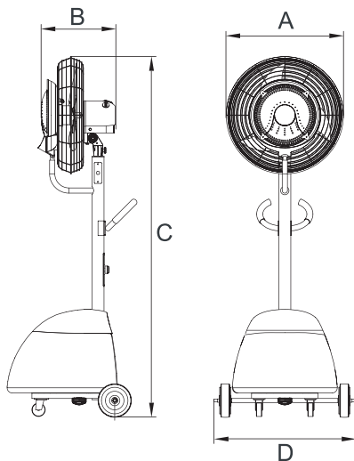
MFS-20
